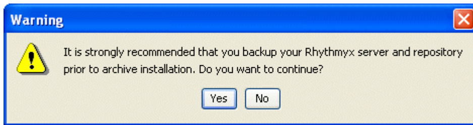
Figure 38: Backup warning
