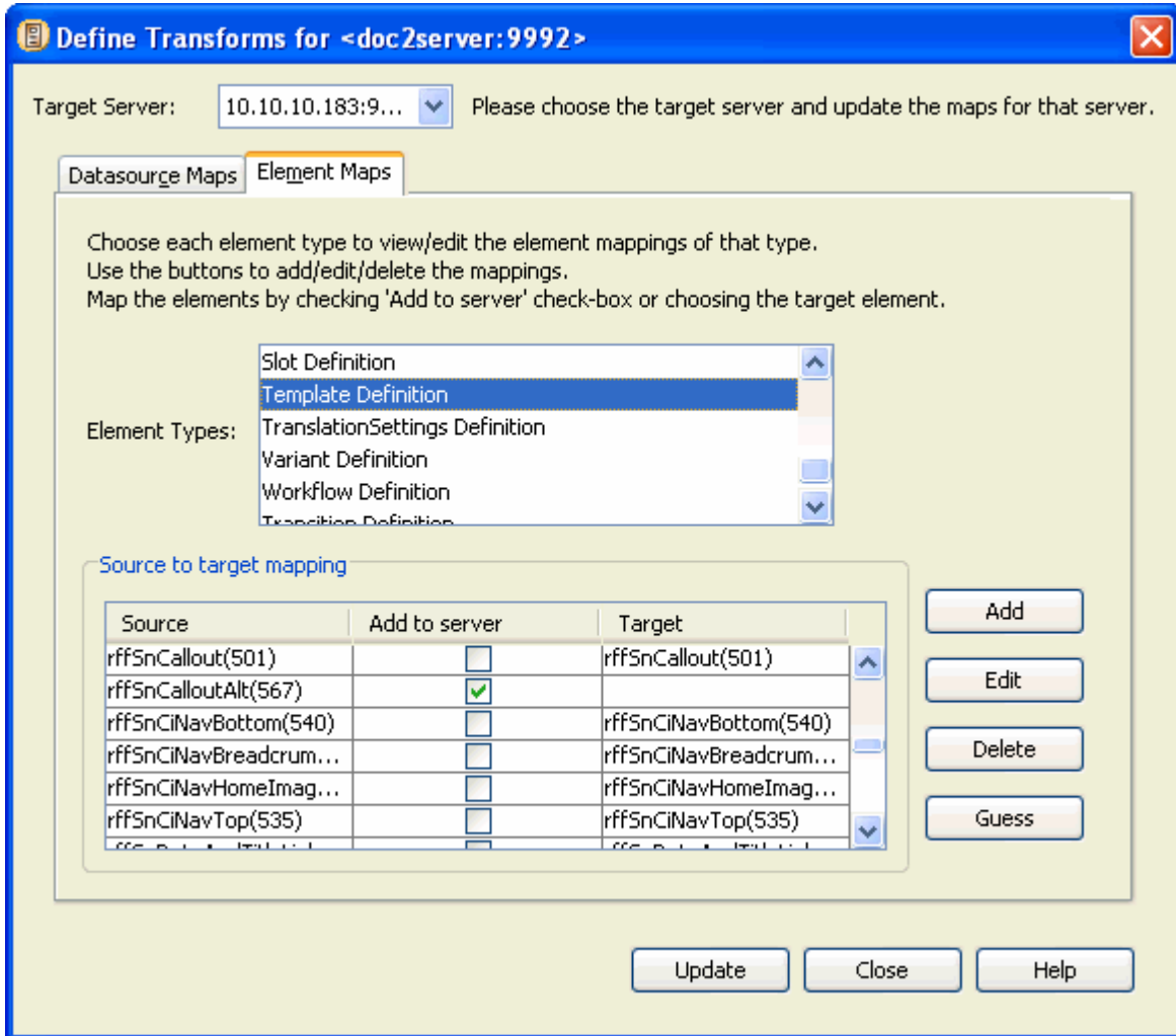
Figure 70: Defining Transforms
