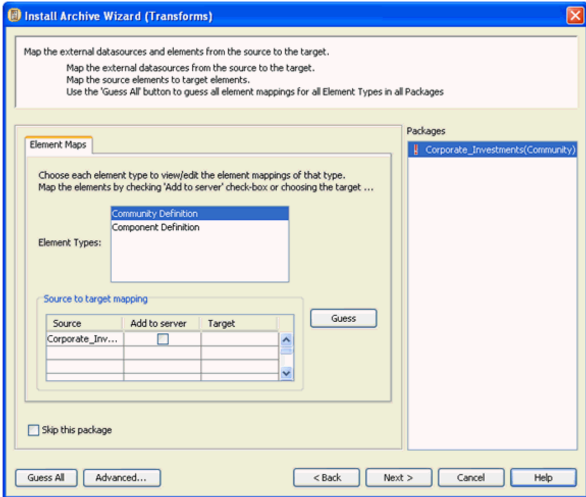
Figure 45: Element Mapping
