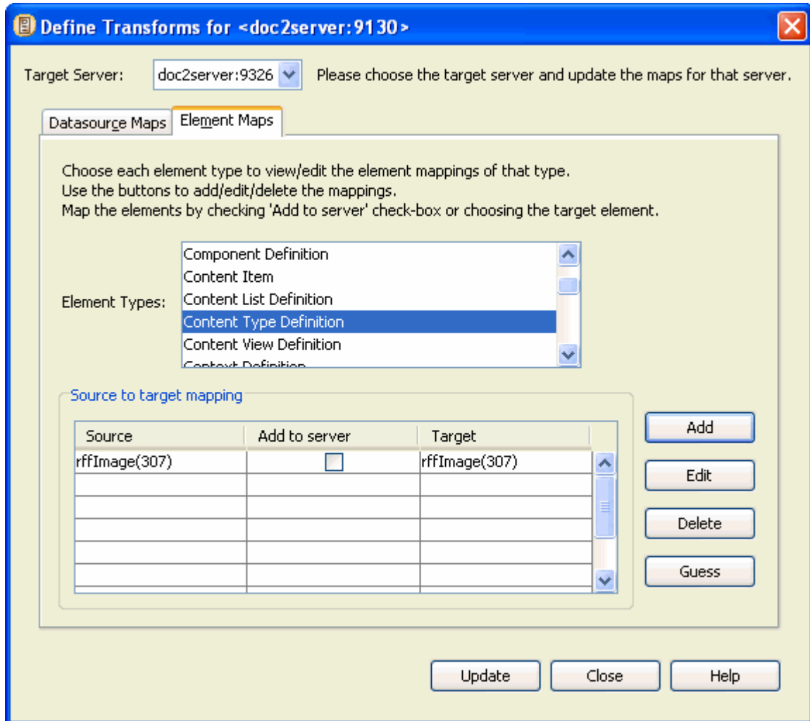
Figure 23: Element mapping
