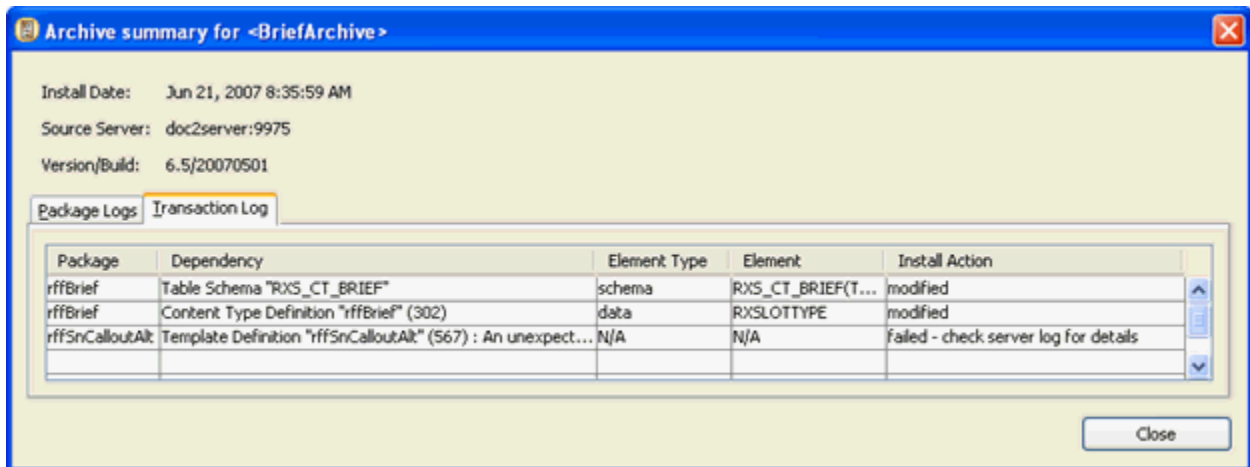
Figure 57: Transaction Log
